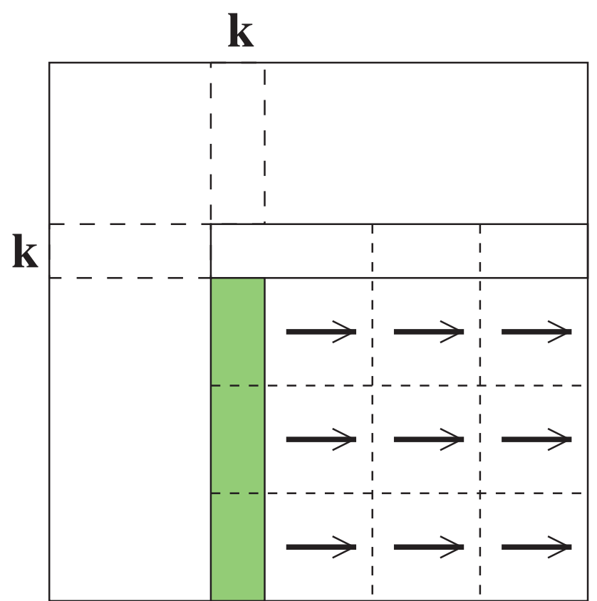
(5a) broadcast of the elimination factors
