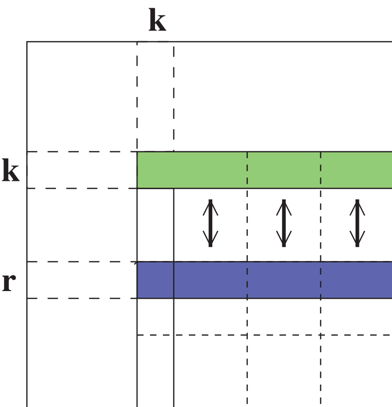
(3) exchange of the pivot row
