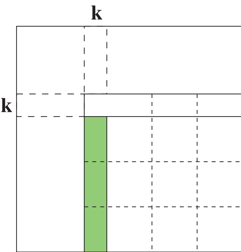
(5) computation of the elimination factors
