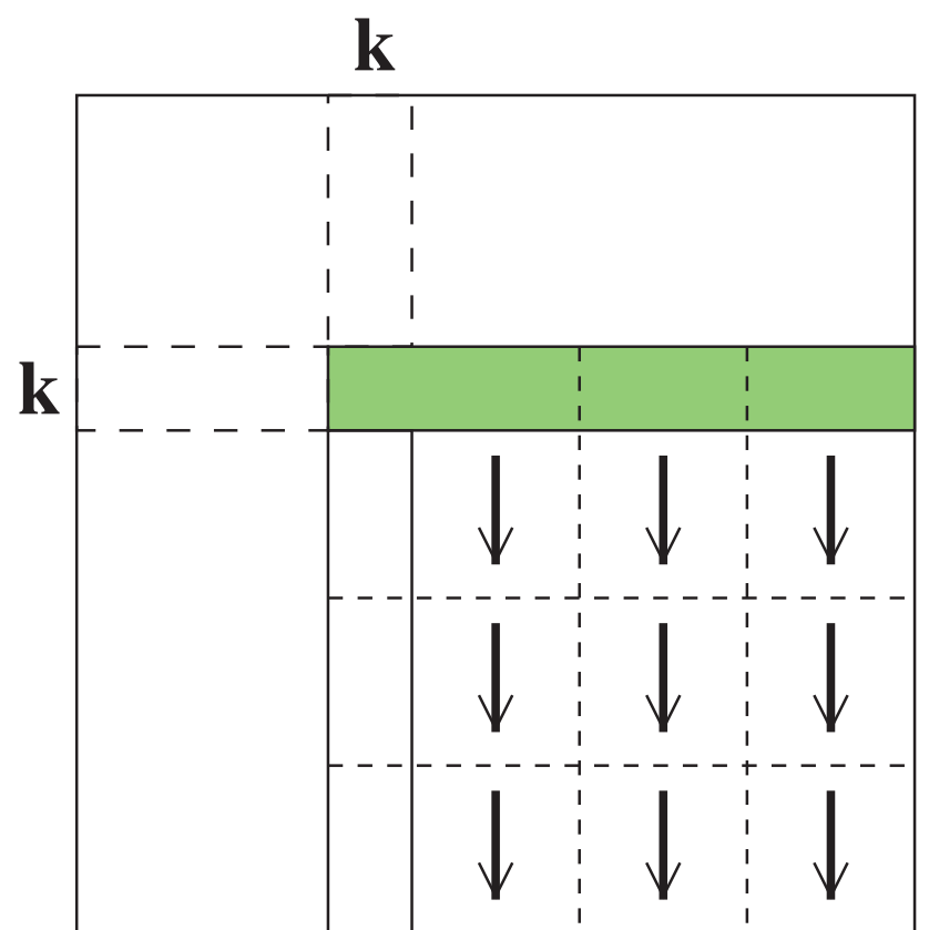
(4) broadcast of the pivot row
