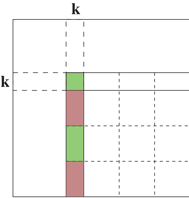
(1) determination of the local pivot elements
