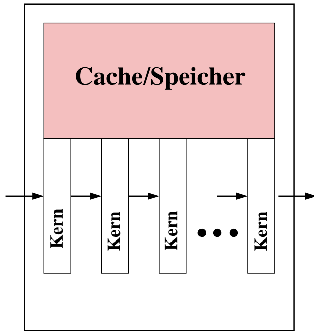
Pipeline-Design
