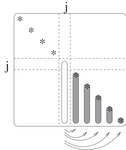
Computation structure for right-looking strategy
