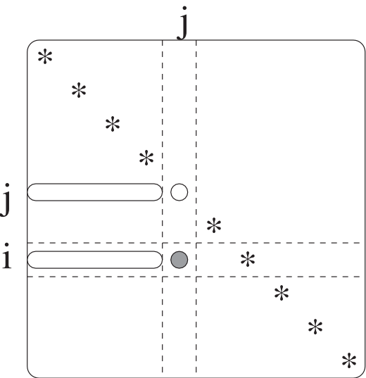
Computation structure for computing l_{ij}
