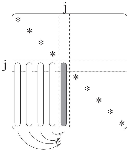
Computation structure for left-looking strategy
