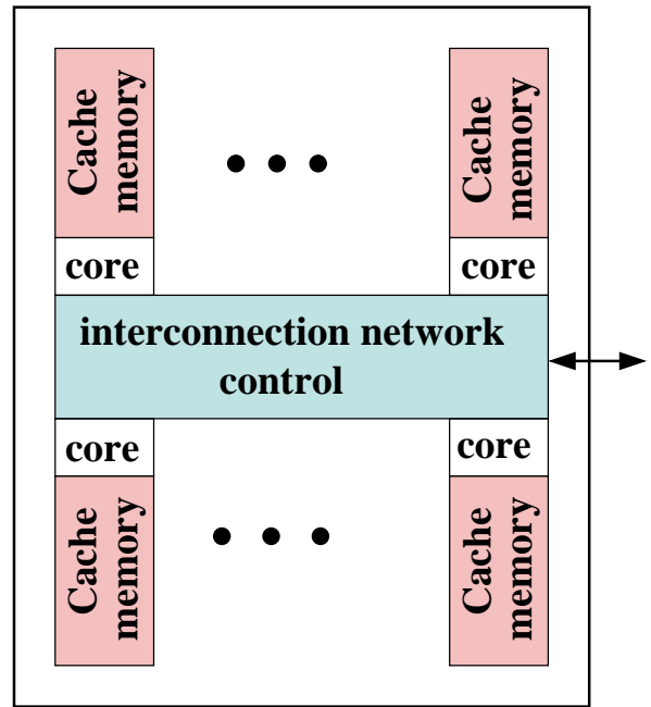
network-based design
