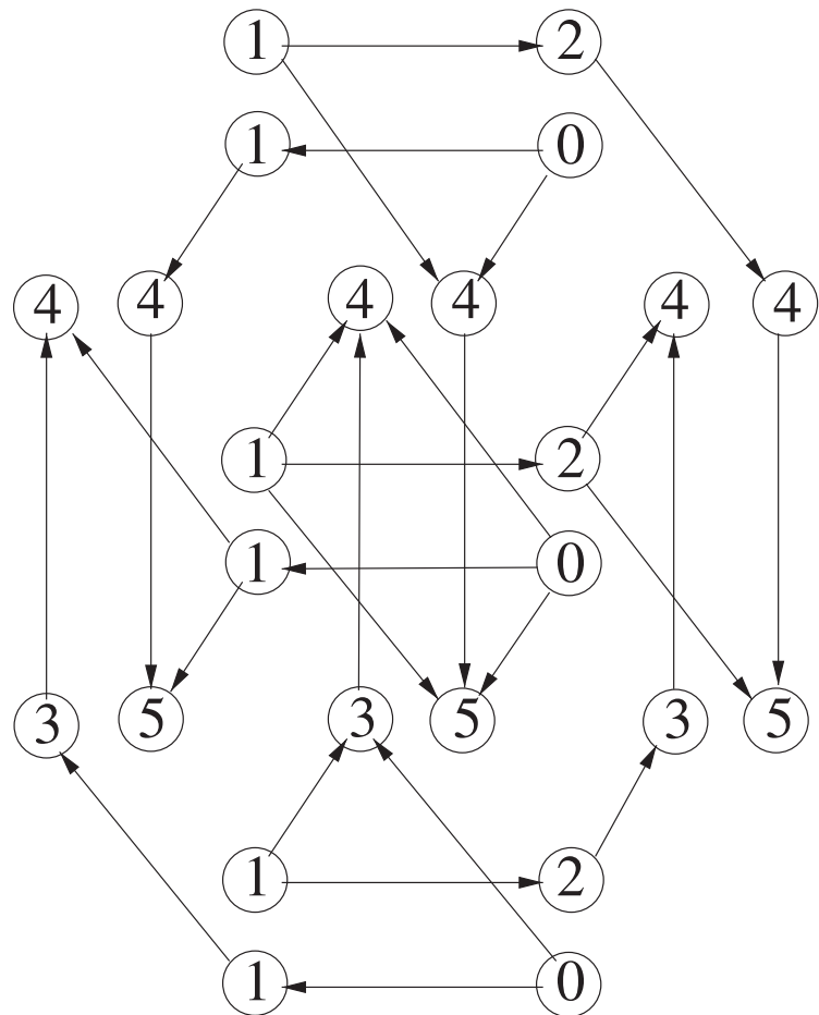
channel dependence graph
